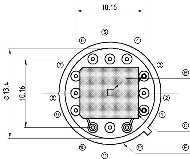
TOP SIDE VIEW (without cap)
